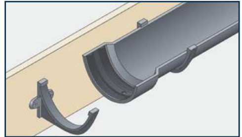
Fig 1. GSP: HYDROSTRIP GUTTER SEALING PACK (N.B. Not suitable for moulded or ogee profiles)
