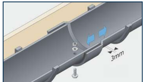
Fig 2. HYDROSTRIP SEALING INSTALL METHOD Illustration of how the specially designed & tested EPDM rubber strips and screws & nuts go together to seal the gutters where they meet.
