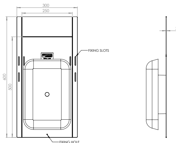
Top Profile
