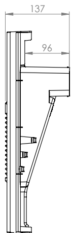
Side Profile
