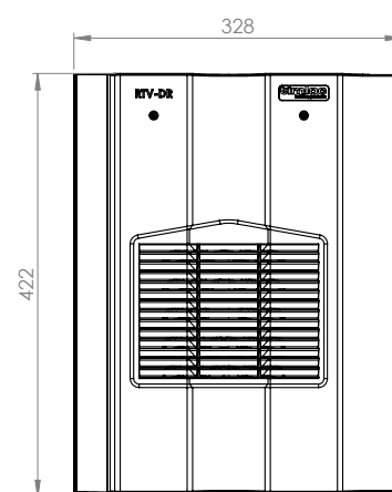
Top Profile
