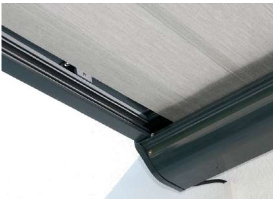
▶ Rear cassette with powerful torsion springs
